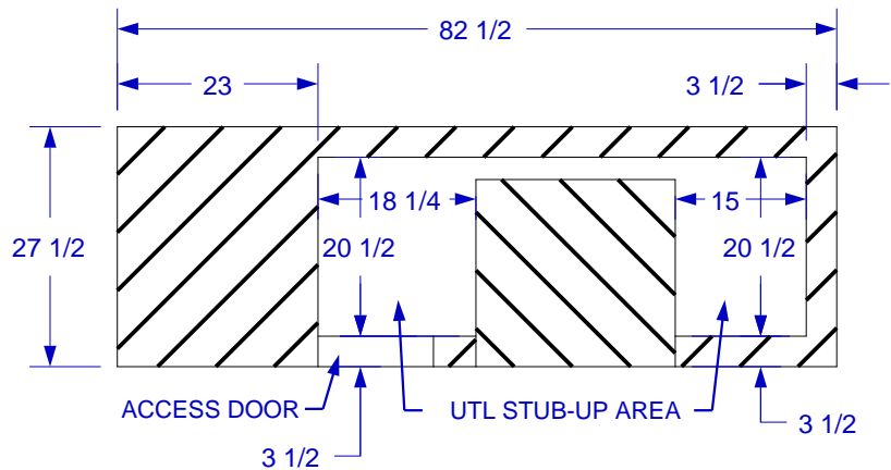
STUB-UP DIAGRAM SCALE 1/2" = 1' 0" (SEE NOTE #2)
