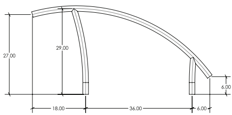
Deck-Mounted Stair Rail
