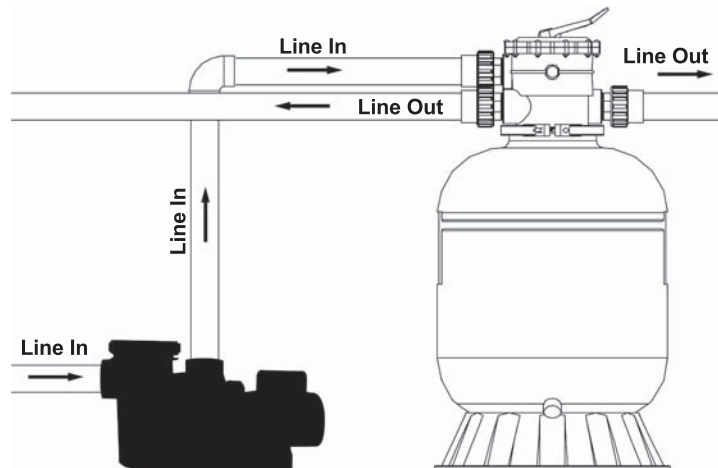
Correct Installation Filter Mounted less than 3' away from pump into the right inlet and water coming from the correct outlet
