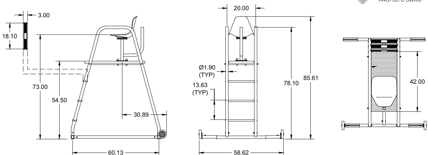
A40703-0 Swivel
